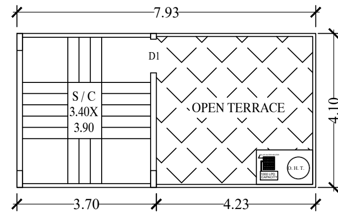
PROPOSED TERRACE FLOOR PLAN
