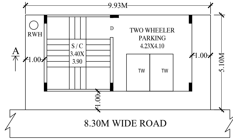
PROPOSED STILT FLOOR PLAN
