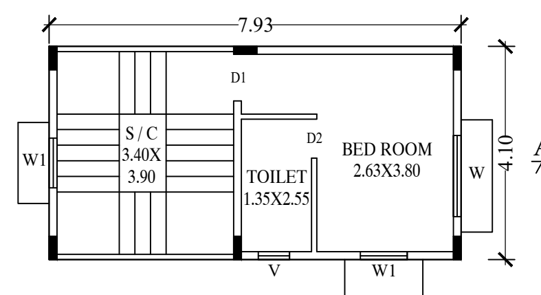
PROPOSED TYPICAL FIRST & SECOND FLOOR PLAN
